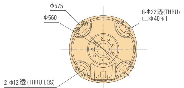
底座安装图 Base installation drawing
